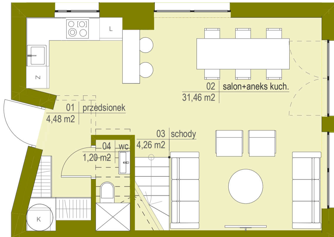
PARTER
