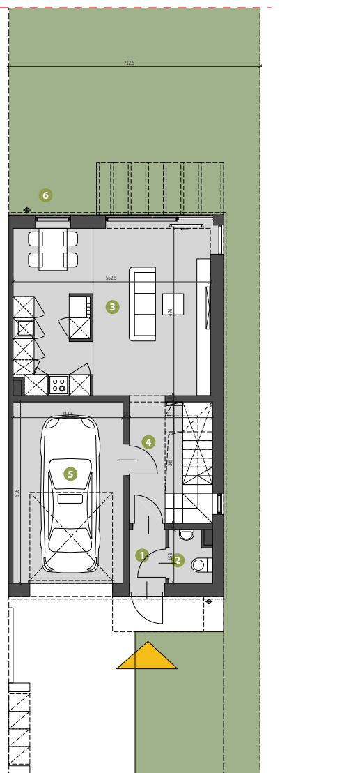
PARTER
