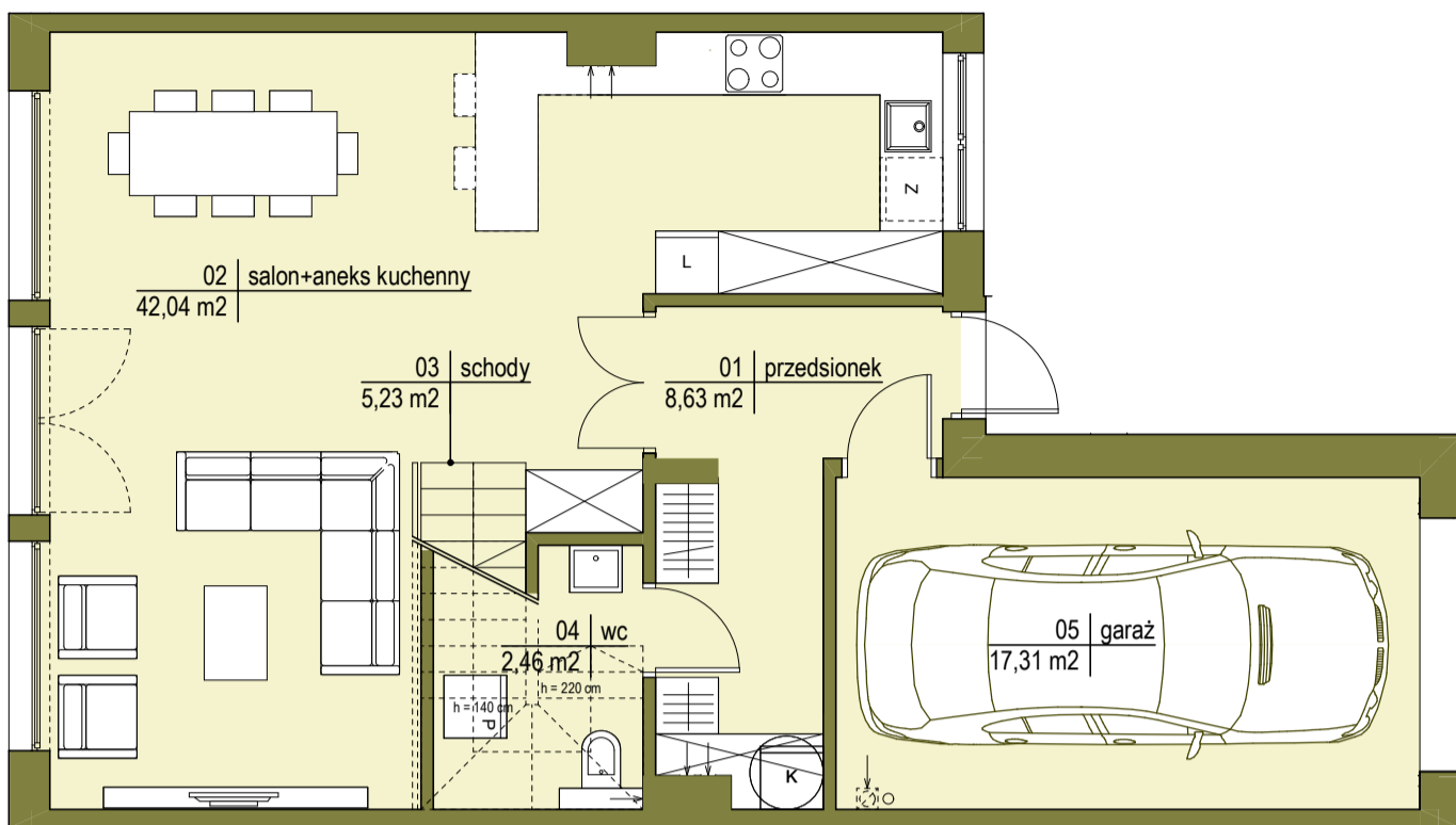
PARTER
