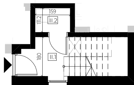
Parter
