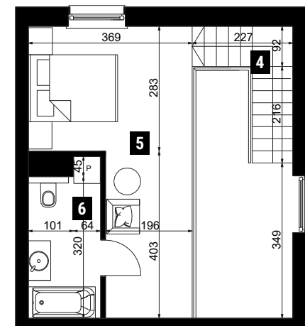
Antresola (+2,80m)
