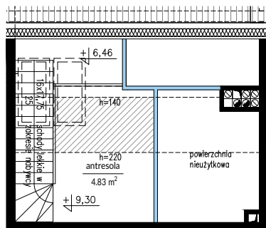
ANTRESOLA
