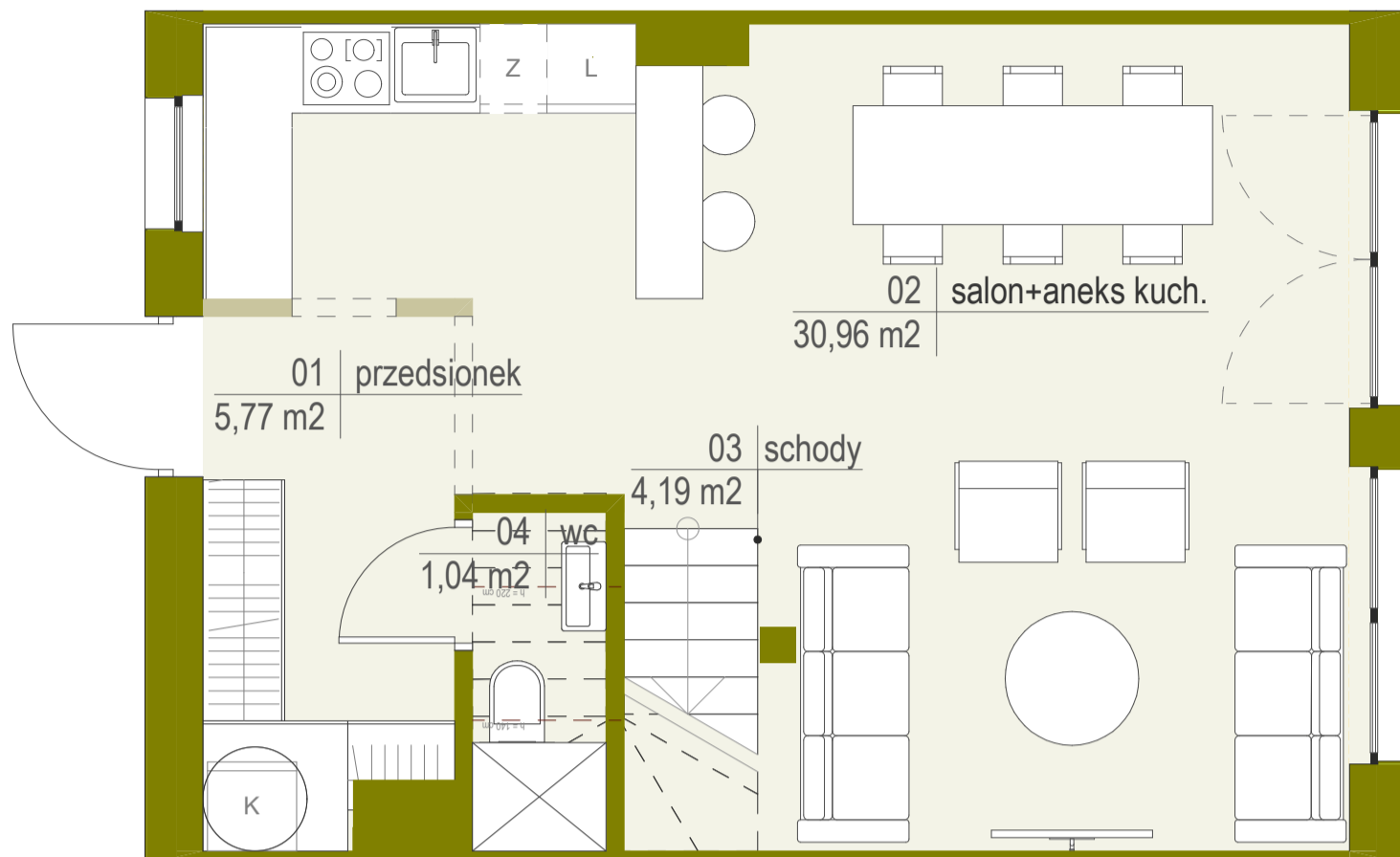
PARTER
