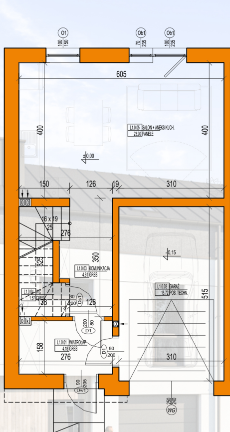
PARTER
