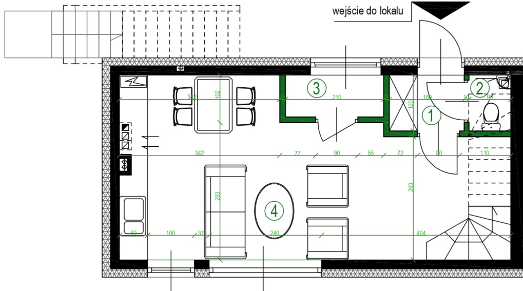
PARTER
