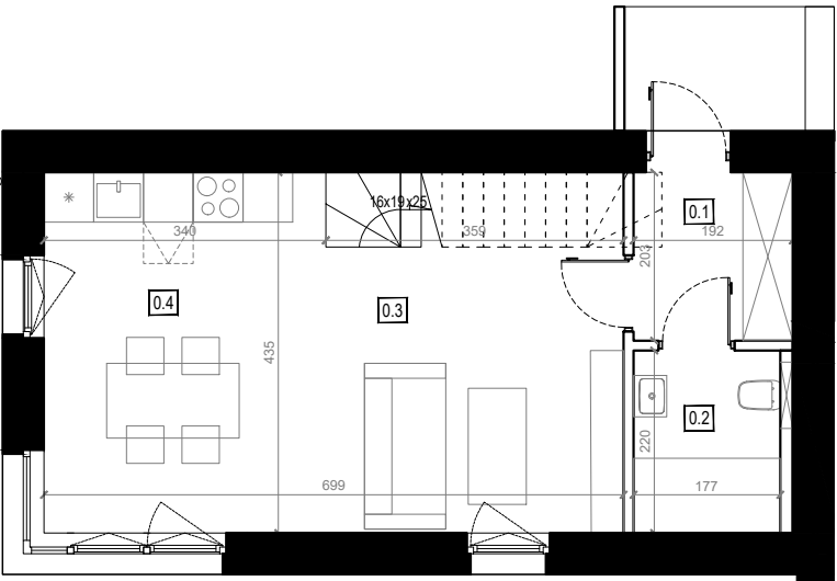
PARTER
