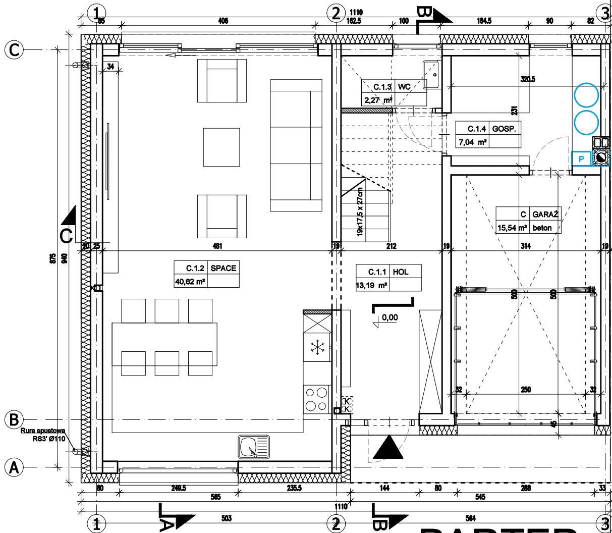
PARTER
