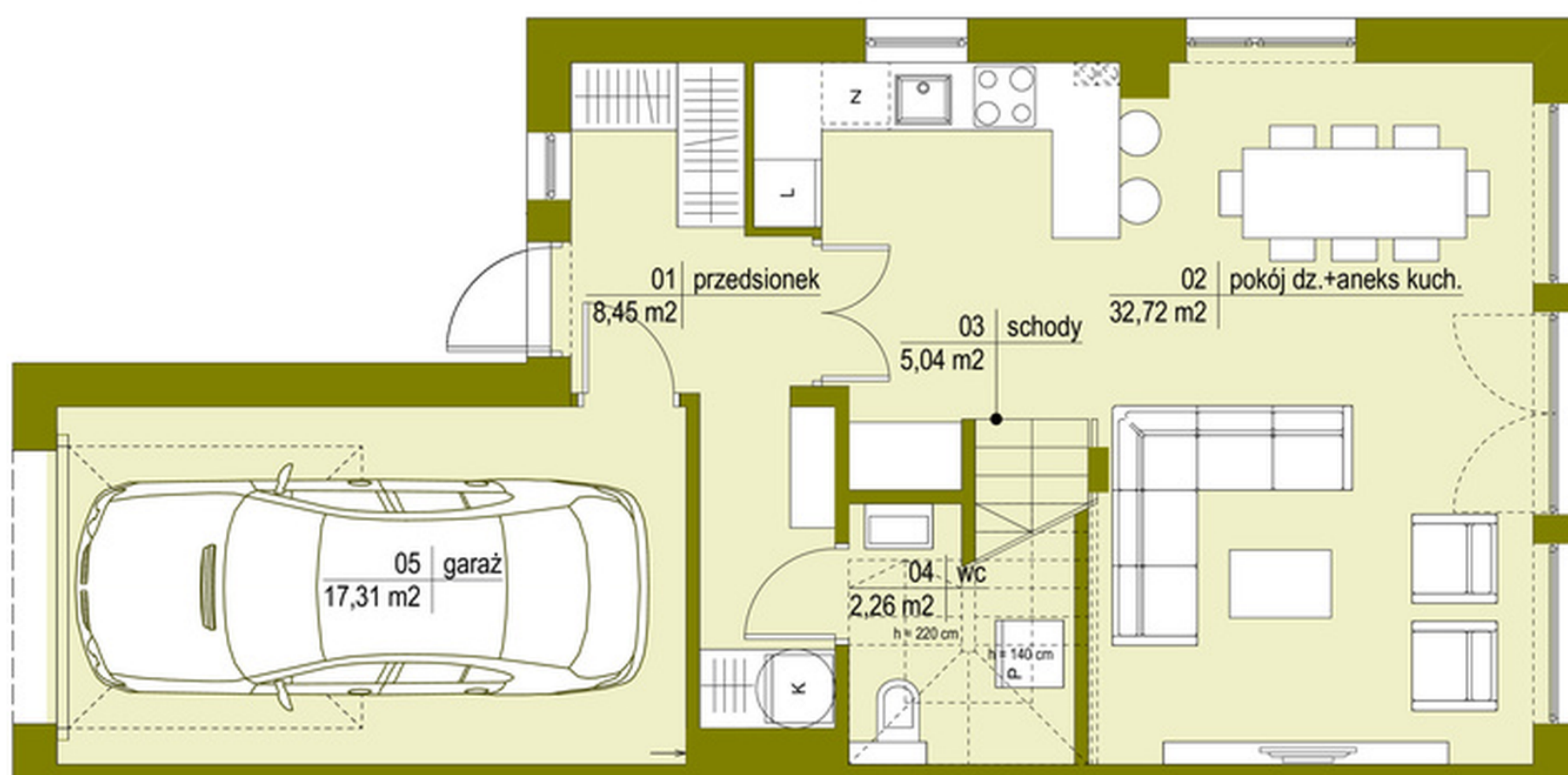
PARTER
