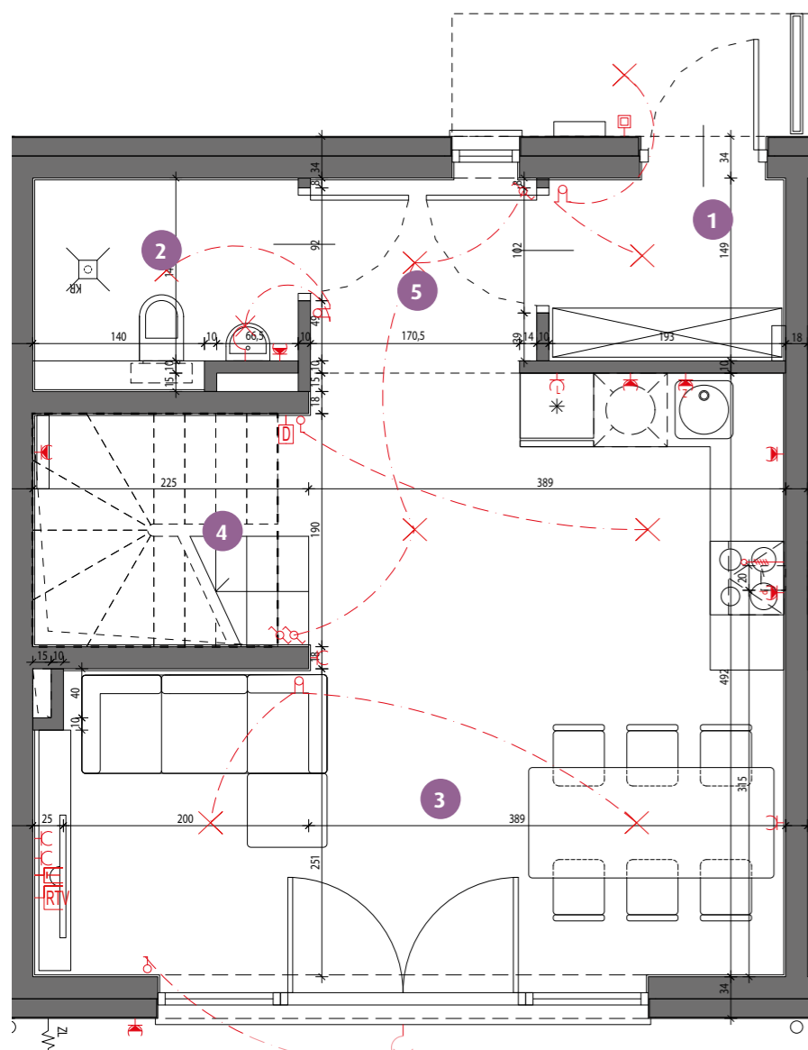
PARTER
